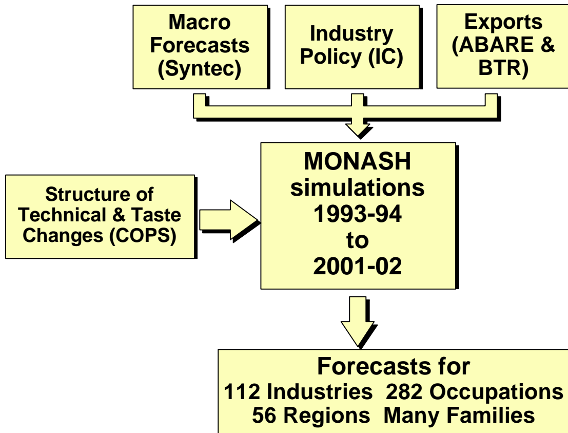
Figure 1: The MONASH Forecasting Methodology
