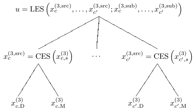
Figure 3: Structure of preferences
